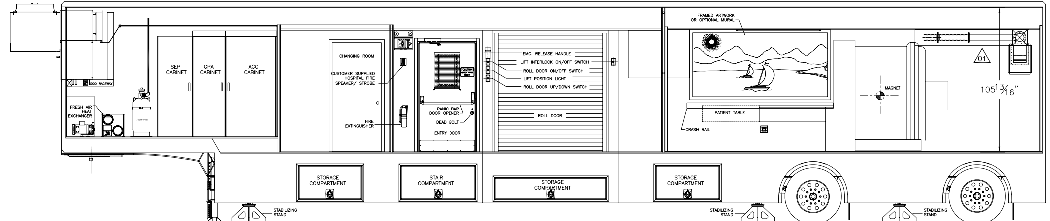
VIEW "B-B" RIGHT SIDE CROSS SECTION
