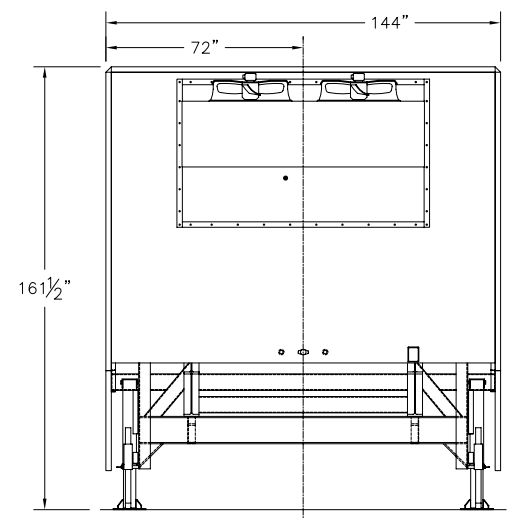
VIEW "C-C" EXTERIOR FRONT VIEW
