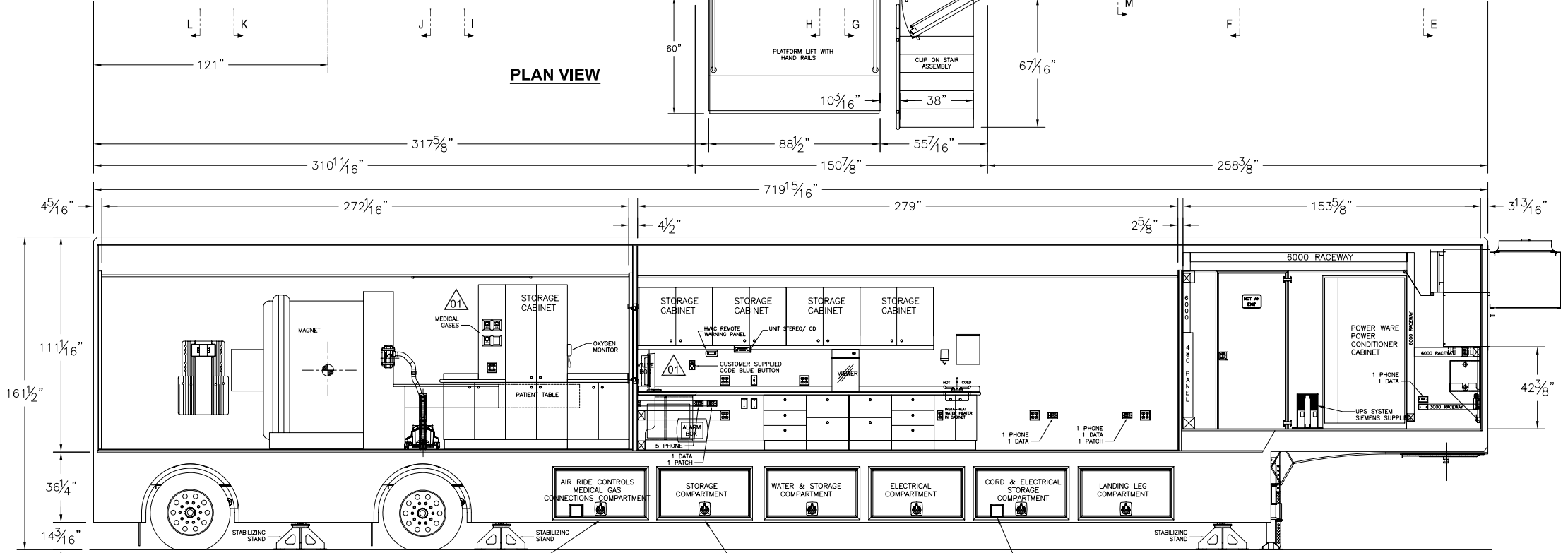
VIEW "A-A" LEFT SIDE CROSS SECTION
