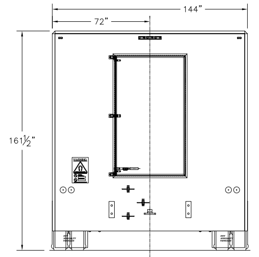
VIEW "D-D" EXTERIOR REAR VIEW
